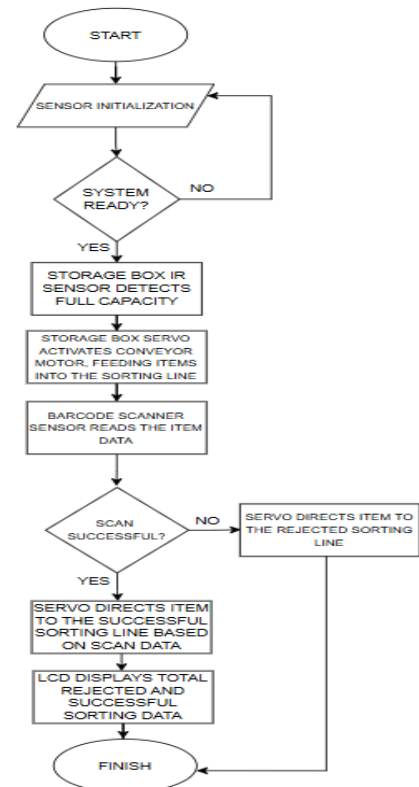
Figure 2. Overall System Flowchart
