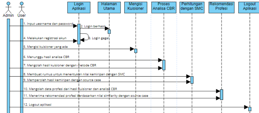
Gambar. 8 Sequence Diagram
