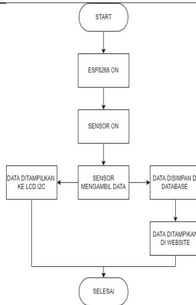
Gambar 8. Flowchart
