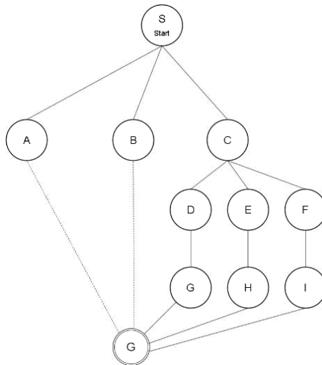
Gambar 3. State Graph
