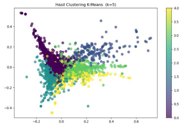
Gambar 5. Plot Hasil Clustering K-means
