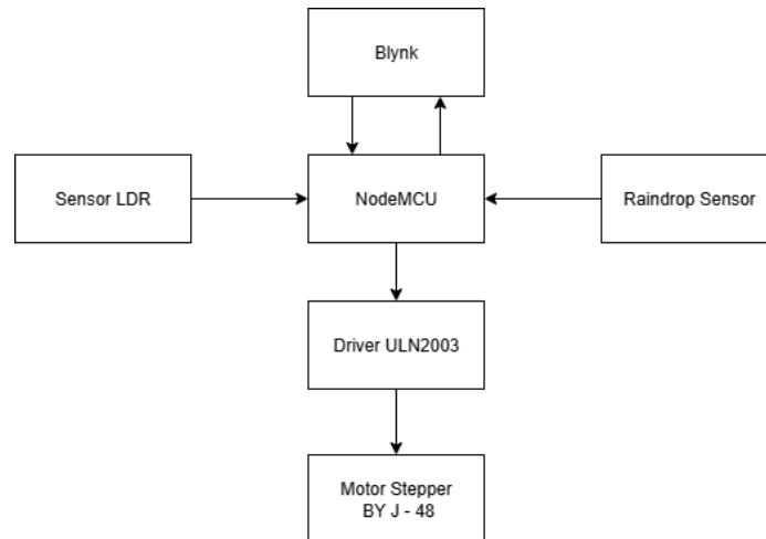
Gambar 5. Diagram Balok
