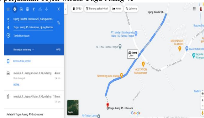
Gambar 13. Halaman Route
