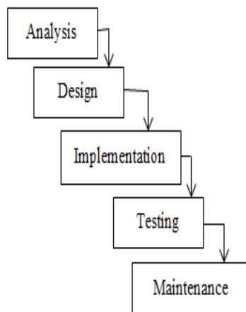
Gambar 1. Model Waterfall
