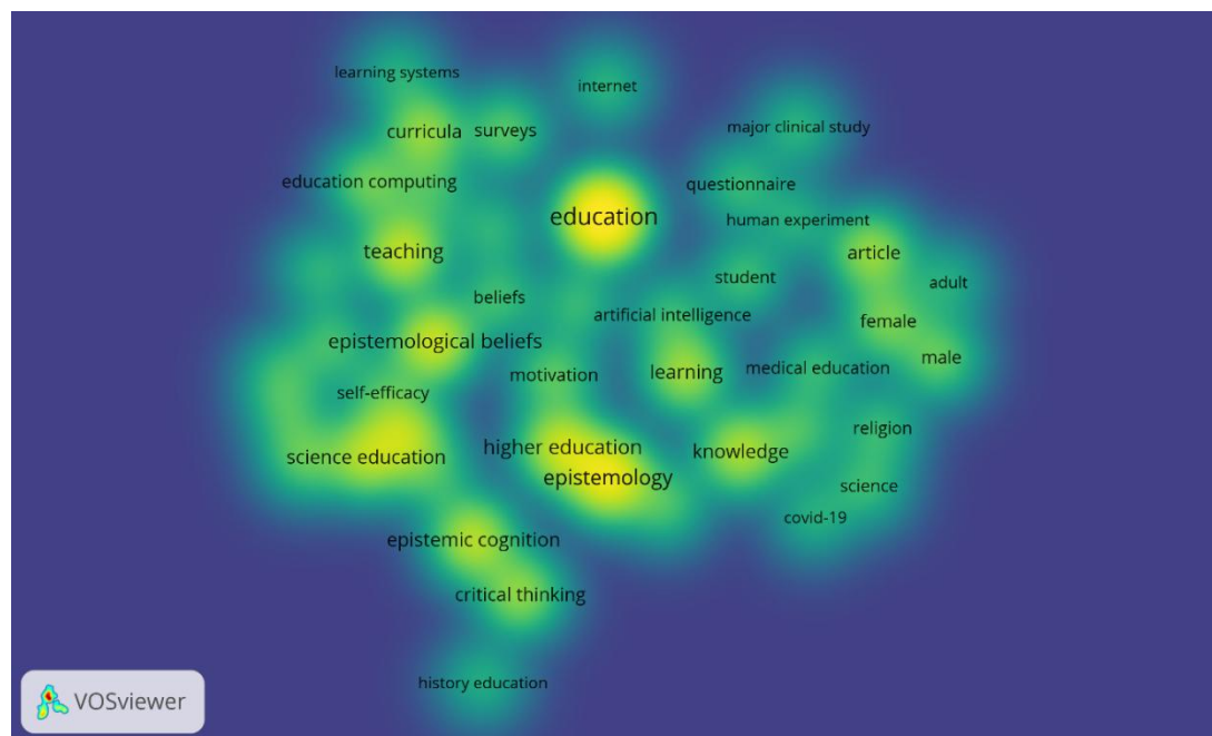
Figure 3. Density Visualization
