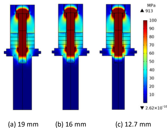
Figure 7 Simulation results of the stress distribution of the transducer with variations in the diameter of the horn at a bolt prestress value of 15 kN.
