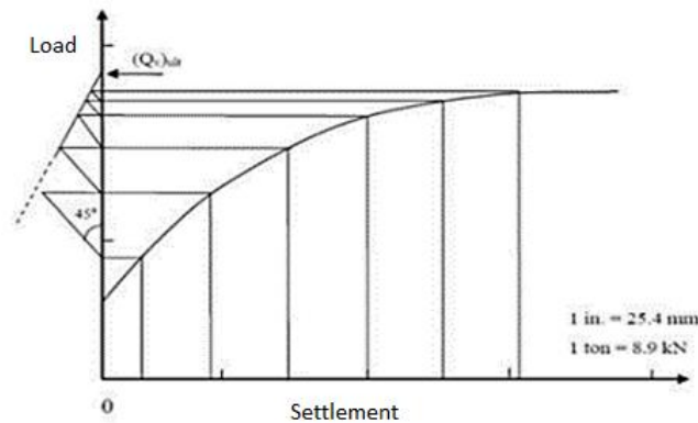
Fig. 3. Mazurkiewics Method Chart
