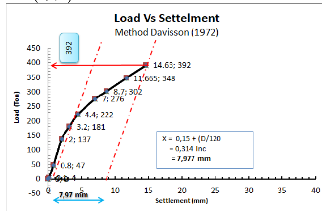
Fig. 9. Interpretation Davisson 's method
