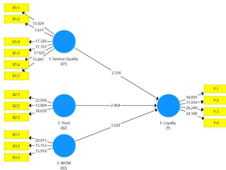
Gambar 1 Boostrapping Test Result
