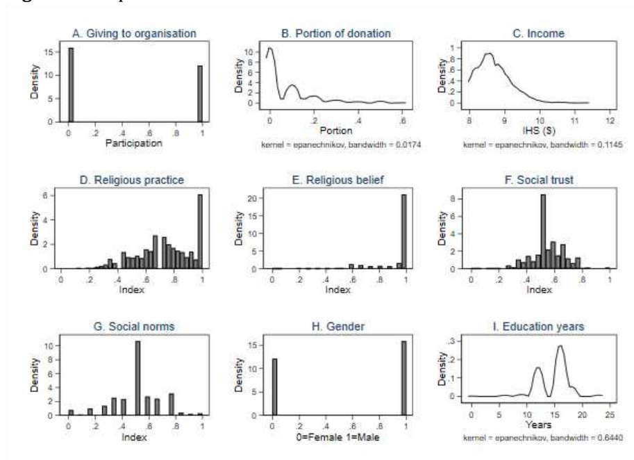
Figure 2. Sample Distribution
