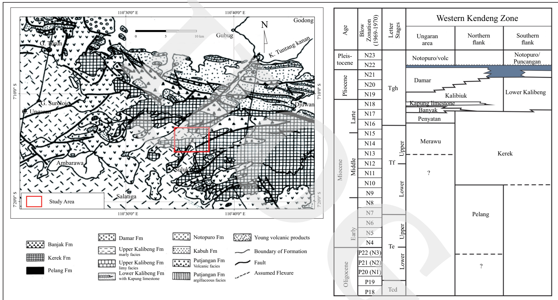
Figure 2. Geological map and general stratigraphy of western Kendeng Zone (de Genevraye and Samuel, 1972). The gas in the studied area leaks through Kerek Formation.
