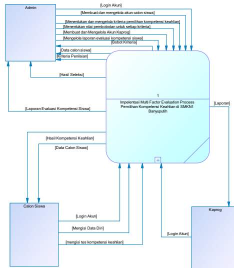
Gambar 2. Gambar Context Diagram
