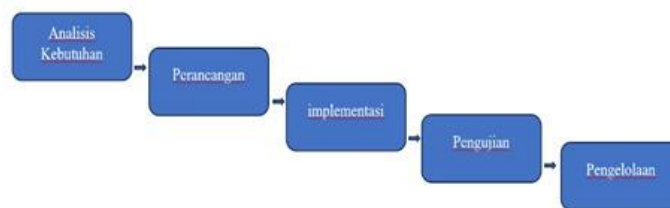
Gambar 1. Gambar Waterfall
