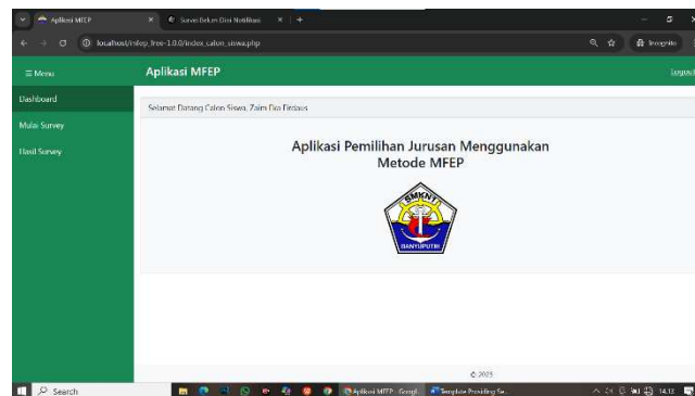
Gambar 12. Dashboard Siswa
