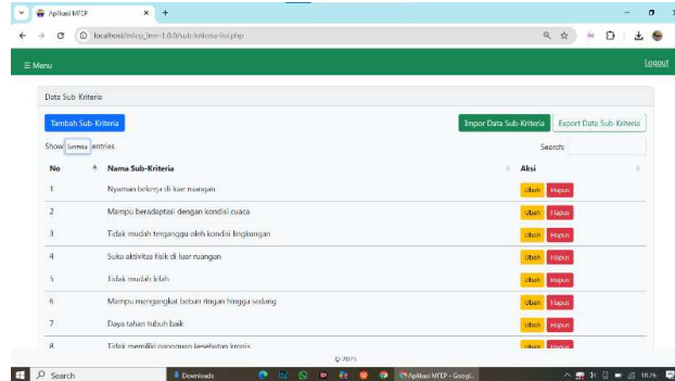
Gambar 10. Sub Kriteria
