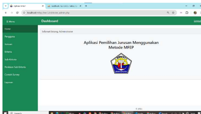
Gambar 6. Dashboard Admin
