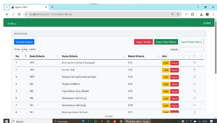
Gambar 9. Kriteria
