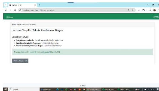
Gambar 14. Hasil Survey
