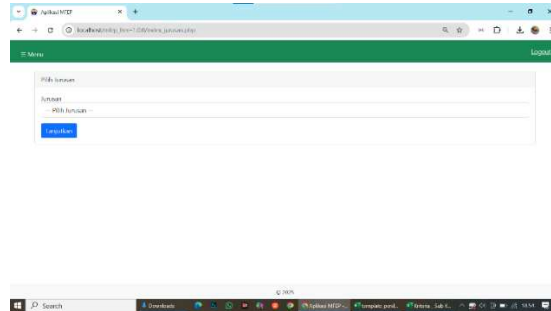
Gambar 13. Halaman Survey
