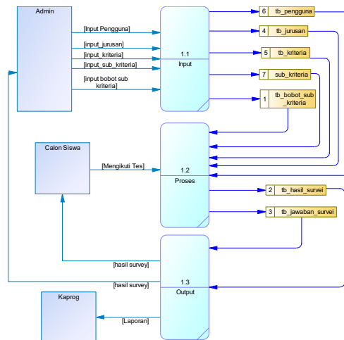
Gambar 3. Gambar Data Flow Diagram
