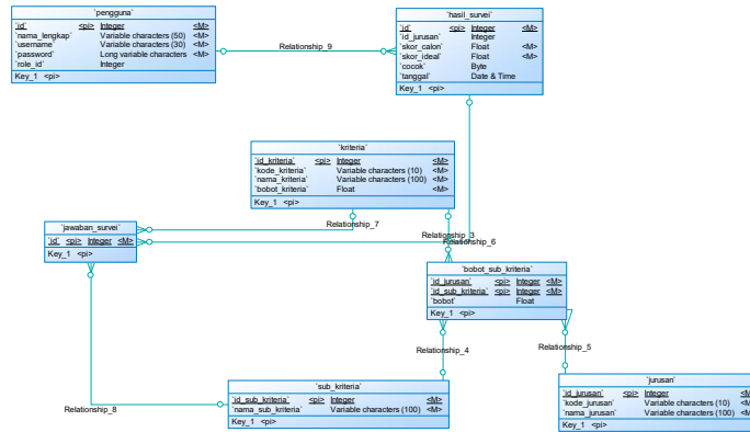
Gambar 4. Gambar Entity Relationship Diagram
