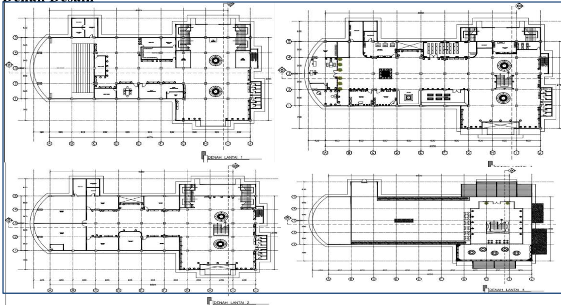
Gambar 8 : Denah Lantai 1-4
