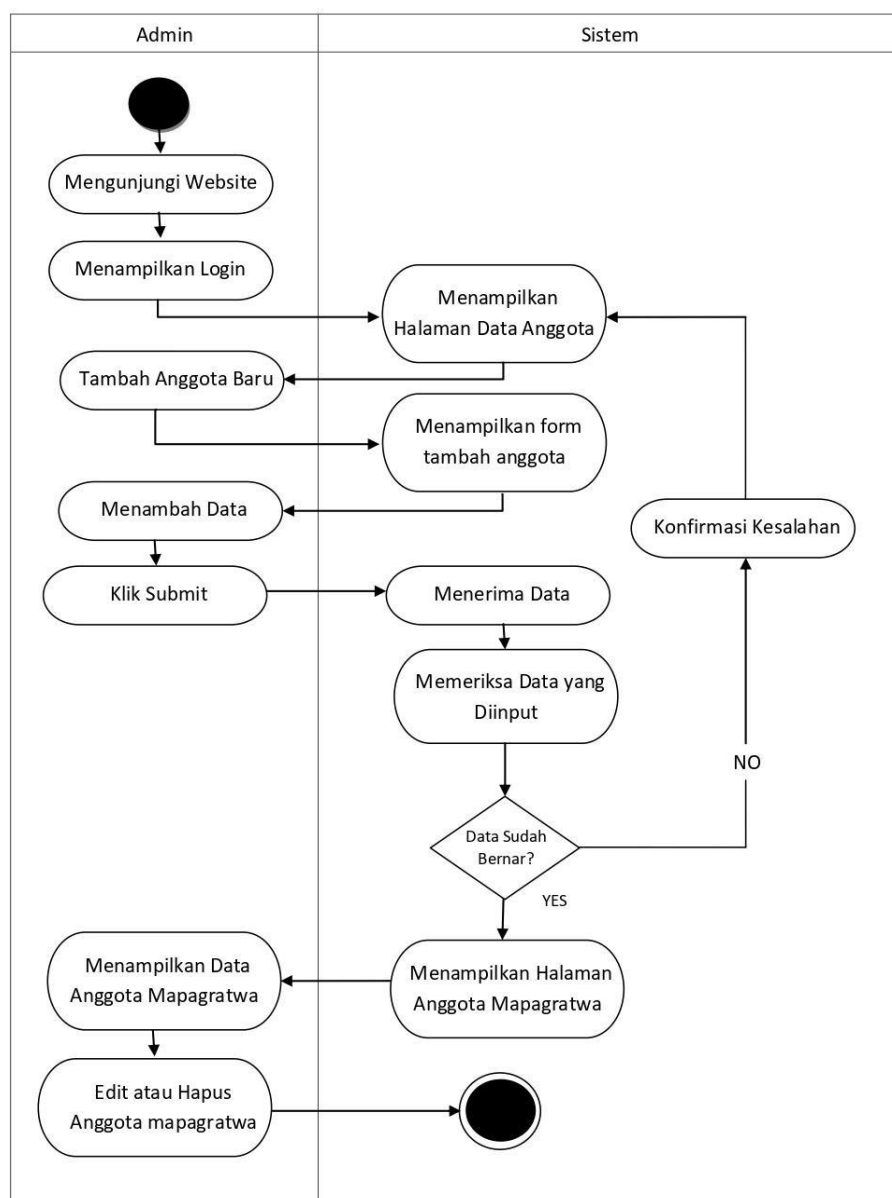
Gambar 3 Activity Diagram Data Manifest Keanggotaan Admin
