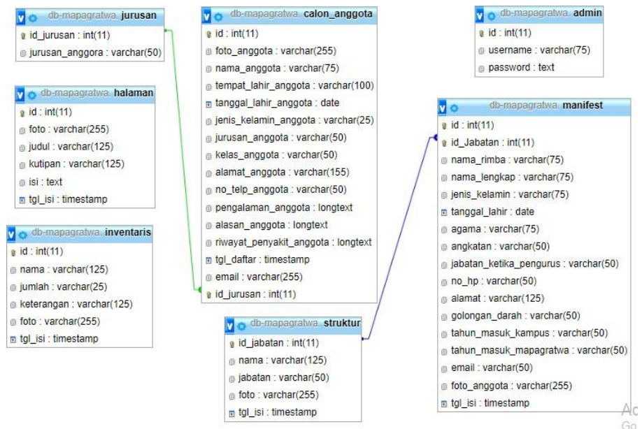
Gambar 4 Desain Class Diagram
