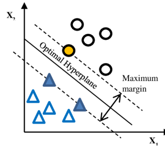
Gambar 2. Margin hyperplane
