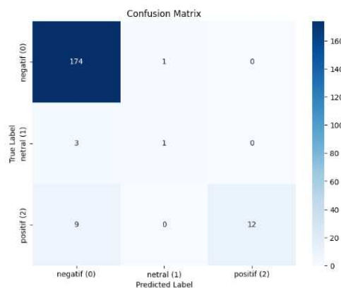
Gambar 8. Random forest
