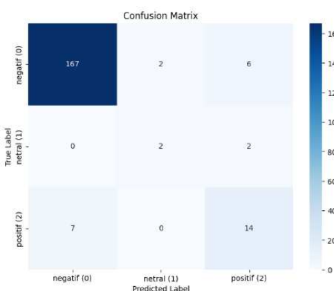
Gambar 9. Decision tree
