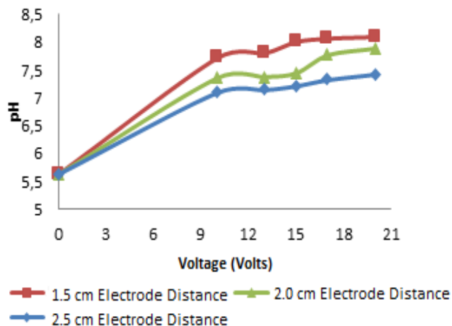
Figure 5. Effect of voltage on the pH value at any variation in electrode spacing
