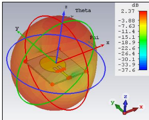
Figure 5. The simulated gain of DGS design
