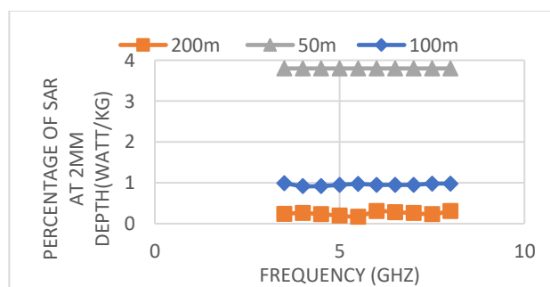
Figure 2. Percentage of SAR at 2 \mu m depth with varying distance from the tower
