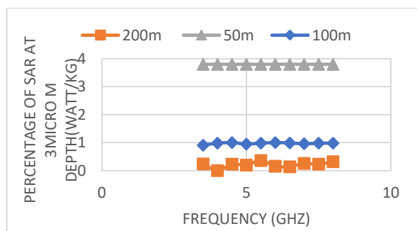
Figure 3. Percentage of SAR at 3 \mu m depth with varying distance from the tower
