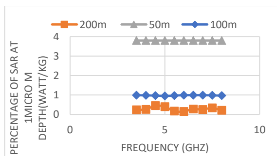
Figure 1. Percentage of SAR at 1 \mu m depth with varying distance from the tower
