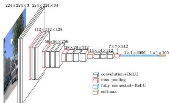
Fig. 5. VGG16 Architectures
