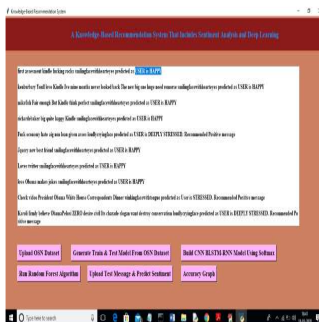
Fig. 9. Each Message Application Detected and Marked.
