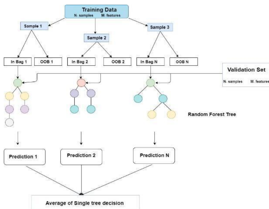
Fig. 3. Architecture Diagram – Diagram Random Forest
