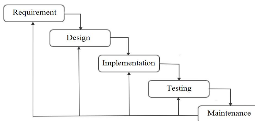
Gambar 1. Waterfall Model
