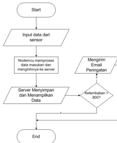
Gambar 4. Flowchart
