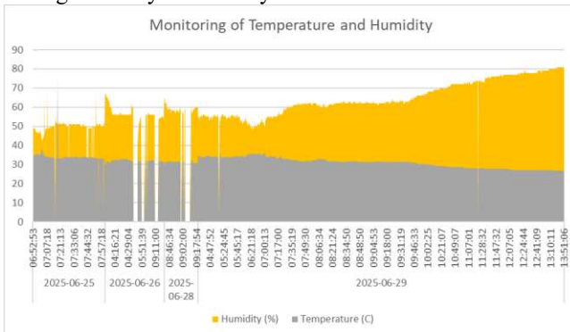
Figure 14. Temperature and Humidity Monitoring Results Graph
