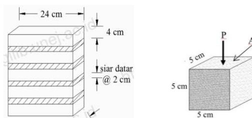
a) masonry prism
