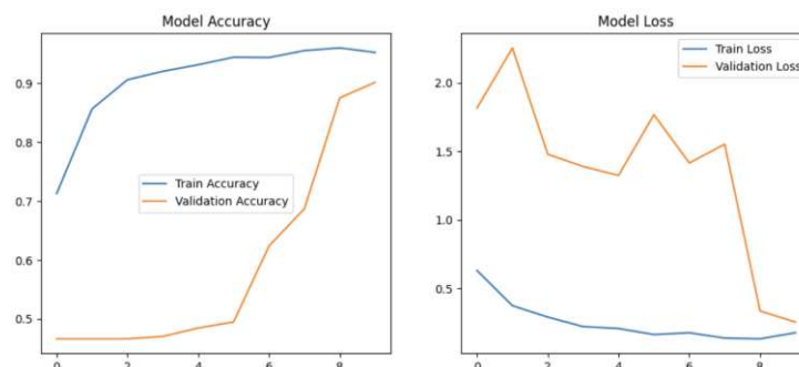
Gambar 4 Training dan Loss Freeze 30 Layer
