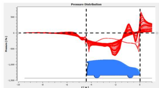
Figure 6. Pressure distribution along with a modeled car with -10^\circ rear spoiler angle
