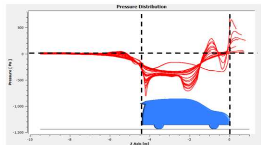
Figure 5. Pressure distribution along modeled car with -20^\circ rear spoiler angle
