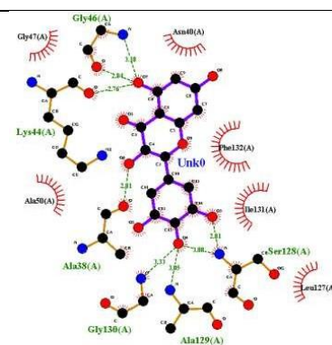
Complex_Redocking_Model1_MYC
