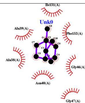
Complex_Redocking_model1_Cineol
