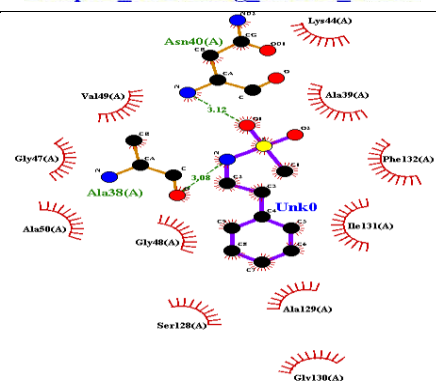
Complex_Redocking_model1_Cineol
