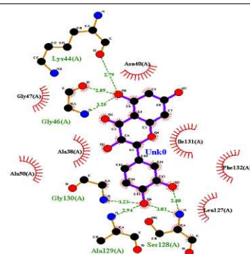
Complex_Redocking_Model1_Que
