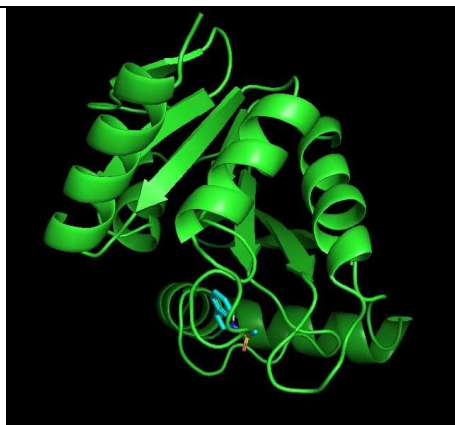
Complex_Redocking_model1_outligan_JFM
