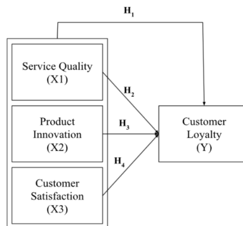
Figure 1. Conceptual Framework
