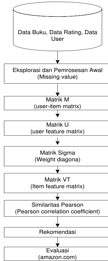
Gambar 1. Alur Penelitian
