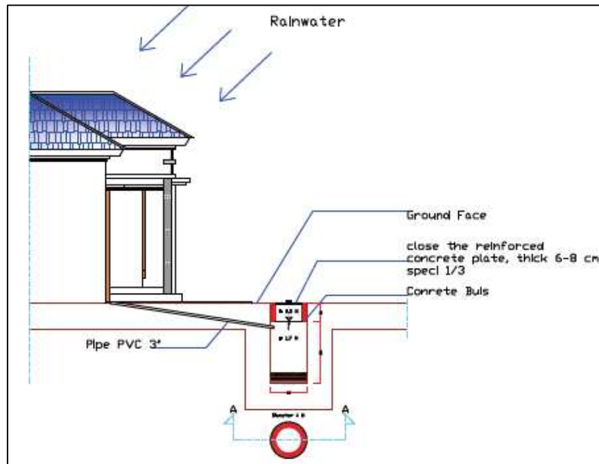
Figure 9. Design of infiltration well [19]
