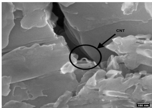
Figure 4. CNT spotted on the surface of BSCCO in 0.2 wt. % CNT addition under 50 K x magnification
