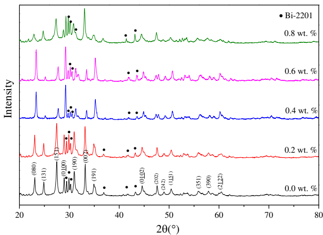
Figure 1. XRD pattern of Bi-2212 with CNT addition of 0.0, 0.2, 0.4, 0.6, and 0.8 wt. %
