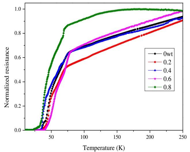
Figure 2. Normalized Resistance versus Temperature of Bi-2212 with CNT addition
