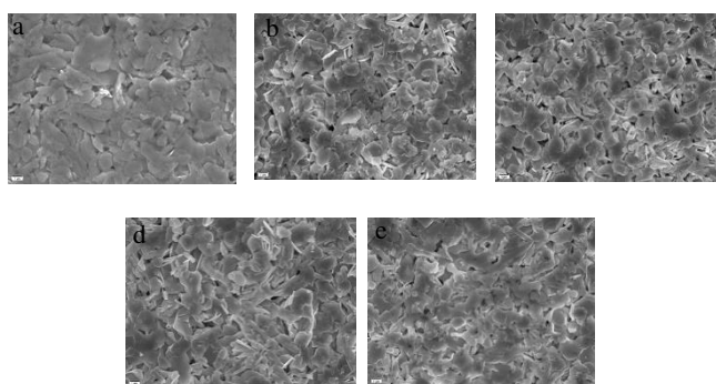
Figure 3. SEM surface morphology of CNT addition to Bi-2212 (a) 0.0, (b) 0.2, (c) 0.4, (d) 0.6, and (e) 0.8 wt. %
