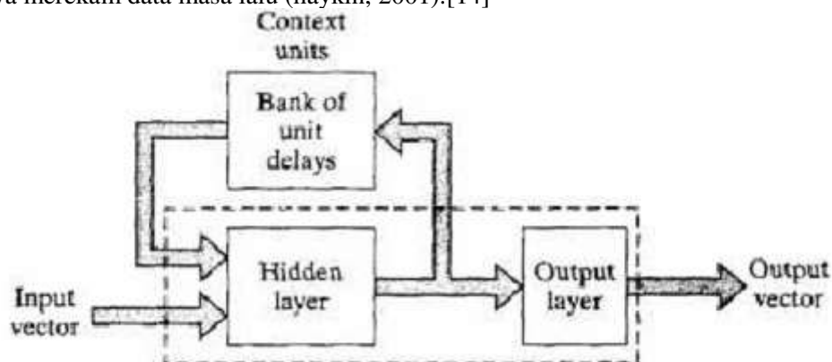
Gambar 2. Arsitektur Simple Recurrent Network Elman (sumber: Haykin, 2001)
