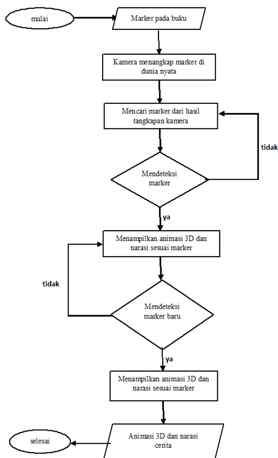
Gambar 2 Alur Sistem flowchart Augmented Reality A Magical Book
