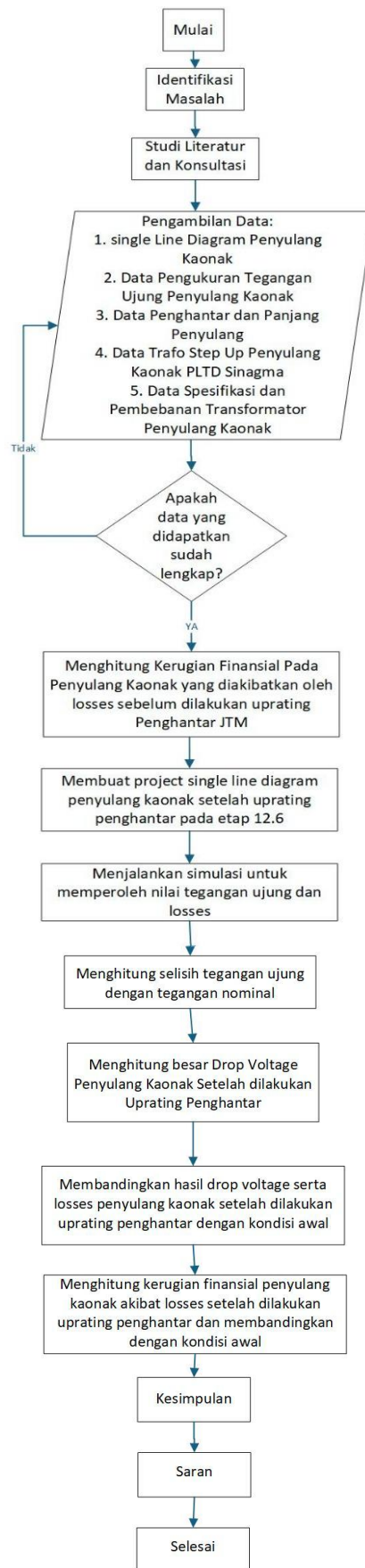
Gambar 1. Flowchart Penelitian
