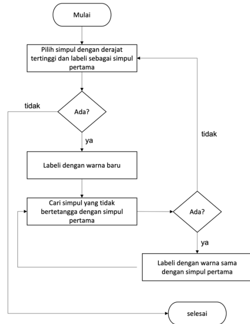
Gambar 2. Algoritma Welch-Powell
