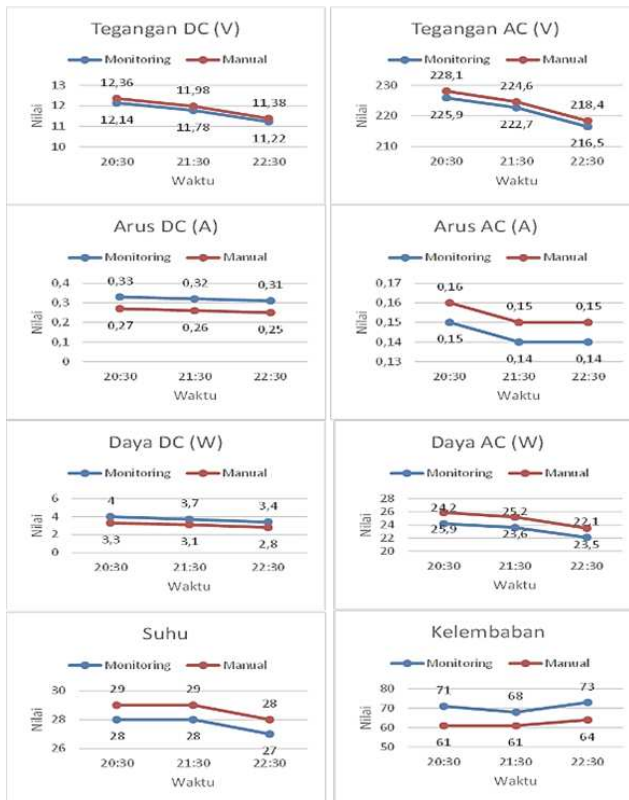
Figure 5: Nighttime Trend Graph of Voltage, Current, Power, Temperature, and Humidity
