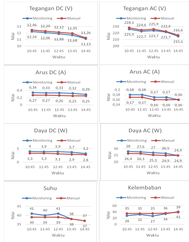
Figure 4: Voltage, Current, Power, Temperature, and Humidity Trend Graph During Daytime
