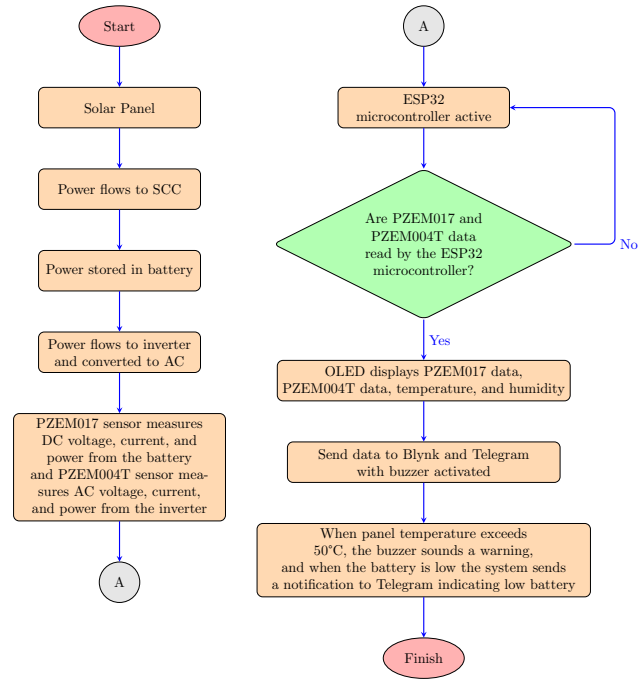
Figure 1: Program Flow on ESP32
