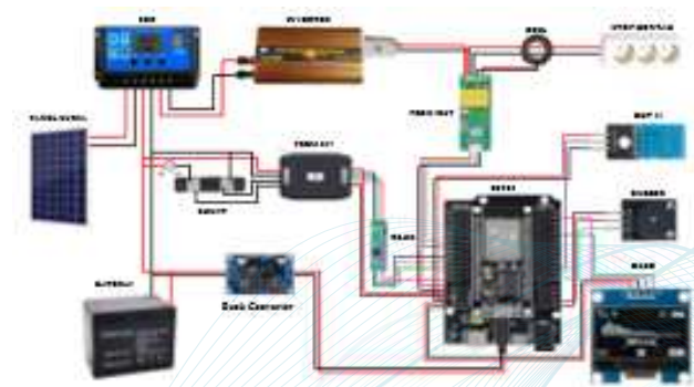
Figure 2: Solar Power Plant Monitoring System Circuit
