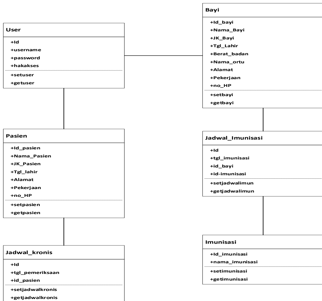
Gambar 3. Class Diagram
