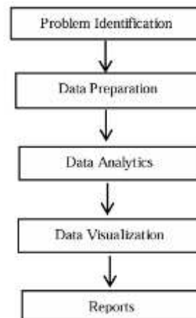
Fig. 1. Research Framework
