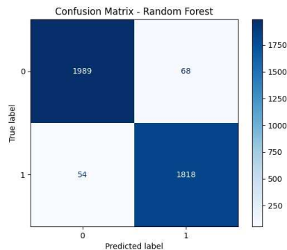
Gambar 10. Confusion matrix
