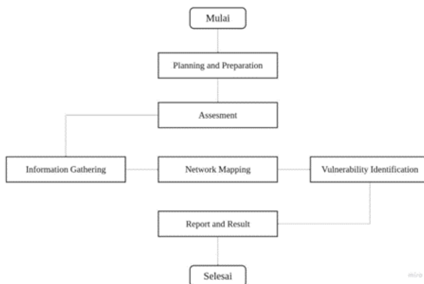
Gambar 1. Alur Penelitian
