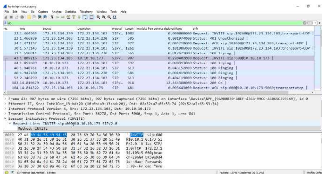
Gambar 19. capture protokol SIP
