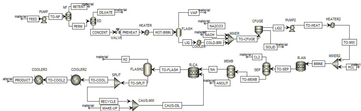
Figure 2. Process simulation of NaOH production from seawater via chlor-alkali membrane process
