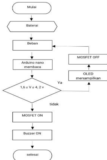
Gambar 4. Flowchart alat
