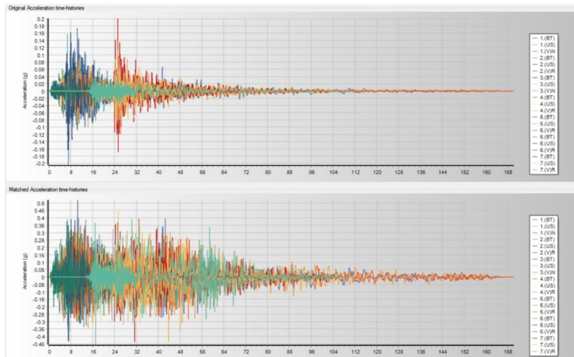
Figure 7. Output of acceleration time histories (Seismomatch)
