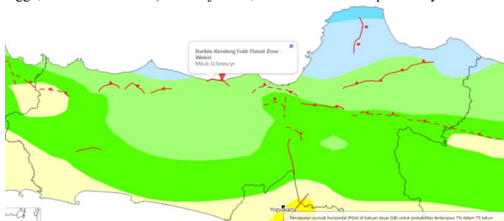
Figure 3. Baribis-kendeng fault
