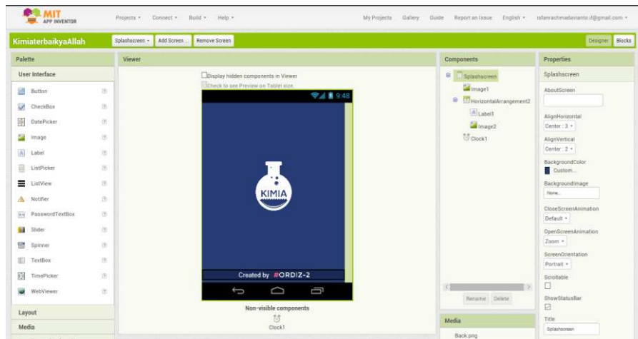
Gambar 3.1 Component Designer
