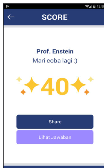
Gambar 4.6 Score Screen
