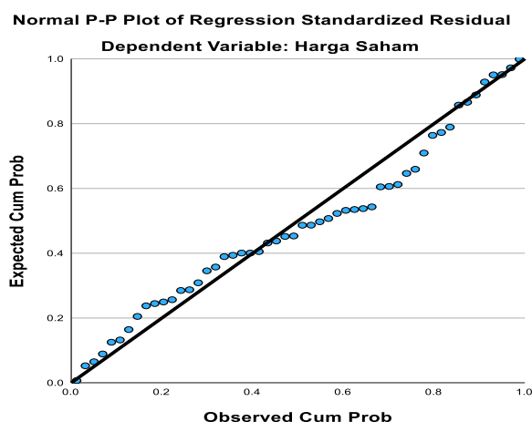
Gambar 1 Grafik Normaly Probability plot.
