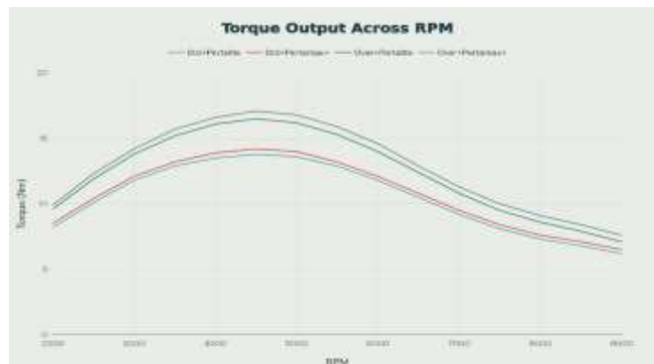
Figure 2. Torque Performance Comparison Across Four Piston-Fuel Configurations
