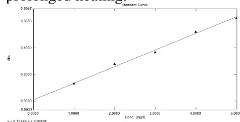
Figure 5. Standard Curve of IC50 Concentration in Antioxidant Test
